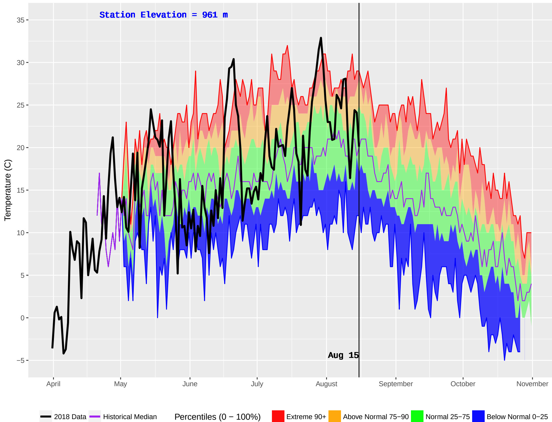
HOLY CROSS 2 (654) : Historical (1998–2016) and Current (2018) Daily Temperature
