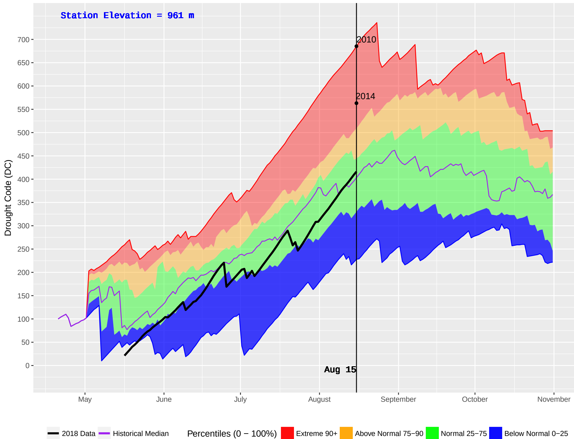
HOLY CROSS 2 (654) : Historical (1998–2016) and Current (2018) Daily Drought Code (DC)
